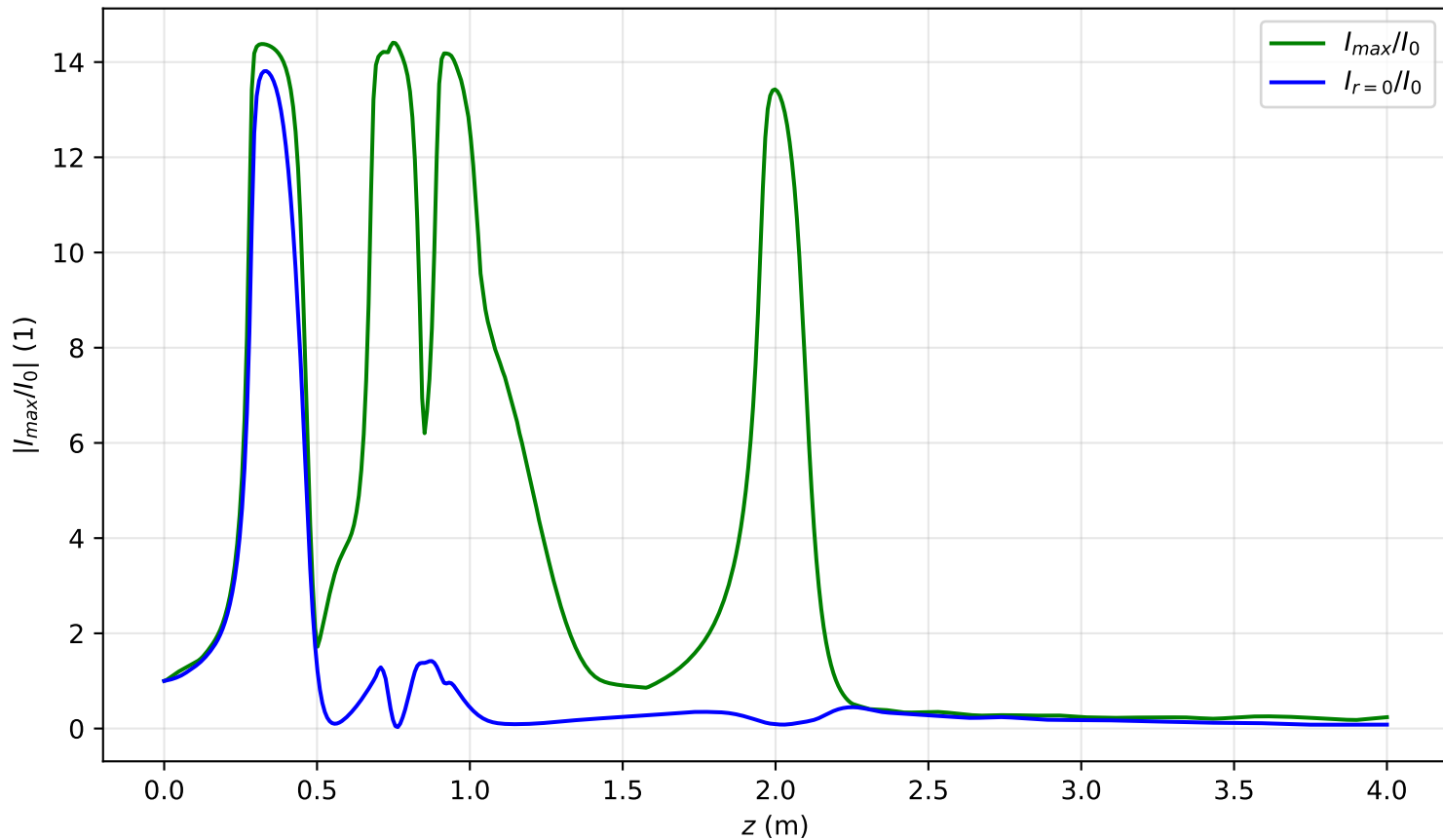
I_{max}(x=0, y=0, z)/I_0 , P_{in}=7.7P_{cr} , noisy input, artificial time
